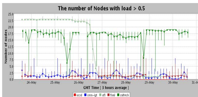
Figure 3. A global plot of the US-CMS farms showing the number of nodes with load higher than 0.5 during a period of one week. These plots are created with the web service repository [14].
